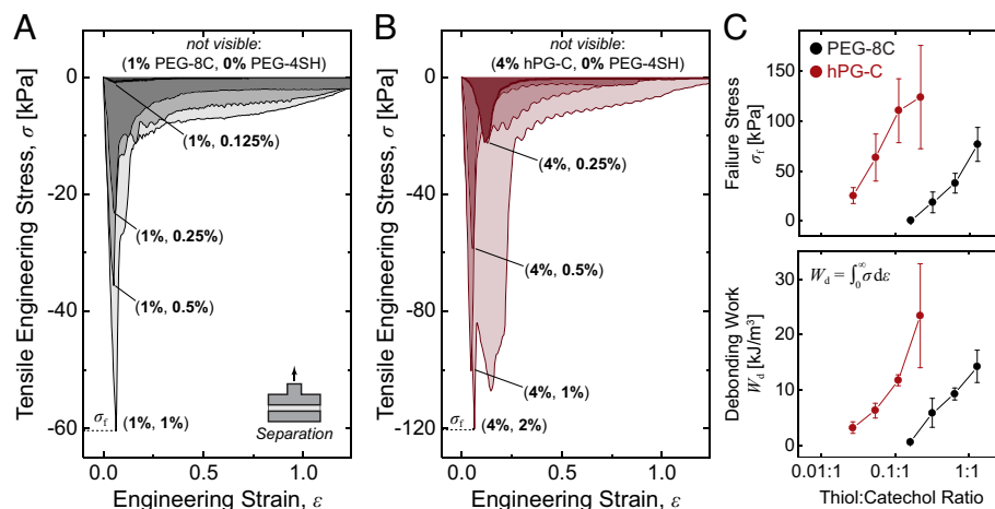
Fig. 3. Adhesion of hydrogels composed of catechol- and thiol-functionalized polymers measured after the gelation shown in Fig. 2. (A) Evolution of the tensile engineering stress \sigma vs engineering strain \epsilon for hydrogels composed of PEG-4SH cross-linked by (A) PEG-8C and (B) hPG-C, where negative stresses correspond to tension. The largest tensile engineering stress is denoted the failure stress \sigma_f , and the integrated area under the stress-strain curve gives the debonding work W_d . (C) Average values of \sigma_f and W_d as a function of the catechol:thiol ratio ( N \geq 3 ); error bars show the SD.
