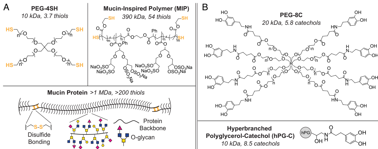
Fig. 1. Schematic overview of the polymers investigated in this work. (A) Thiol-functionalized polymers and (B) catechol-functionalized cross-linkers. The structures shown are ideal; the average functionalization of thiol or catechol groups per molecule is stated in the image labels.
