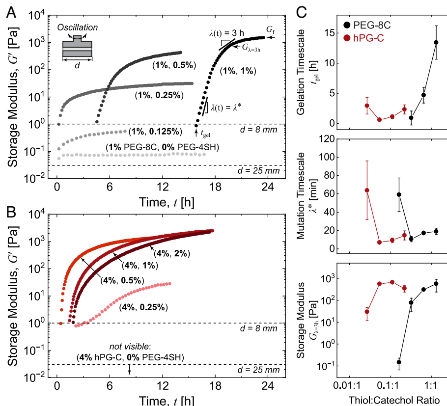
Fig. 2. Gelation dynamics of catechol- and thiol-functionalized polymers. Evolution of the storage modulus G' vs time t at frequency \omega = 5 rad/s for (A) 1% PEG-8C, 0 to 1% PEG-4SH, 0.16 mg/mL tyrosinase and (B) 4% hPG-C, 0 to 2% PEG-4SH, 0.64 mg/mL tyrosinase. The dashed lines show the minimum measurable moduli for different parallel plate test fixtures (diameter d = 8 or 25 mm). The gelation timescale t_{gel} , fastest mutation timescale \lambda^* , storage modulus G_{\lambda=3h} , and final storage modulus G_f are indicated. (C) Average values of t_{gel} , \lambda^* , and G_{\lambda=3h} as a function of the thiol:catechol ratio ( N \geq 3 ); error bars show the SD.
